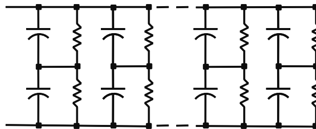
Series - parallel array, no center connection
