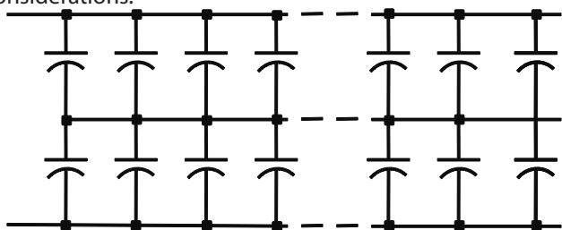
Parallel-series array with common center connection
